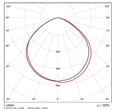
Photometric curve 1SP SPF20W*
