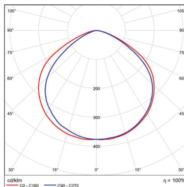
Photometric curve 1SP SPF10W*
